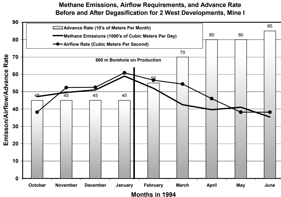
Figure 4. Methane emissions and section advance rates for the 2 West gate entries prior to and after development of a methane drainage shield borehole at one of Minales Monclova's mines in northern Mexico.
