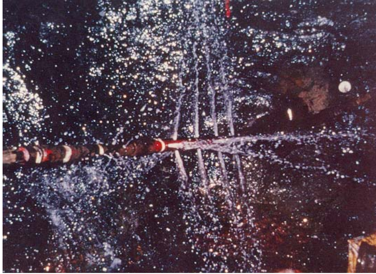
Figure 9. Straddle packer used by REI Drilling, Inc. to hydraulically fracture directionally drilled boreholes at the Soldier Canyon Mine.
