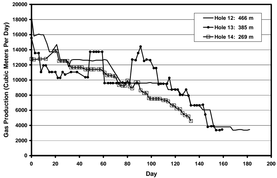
Figure 3: Average Daily Gas Production from Three Boreholes Drilled in Mine I
